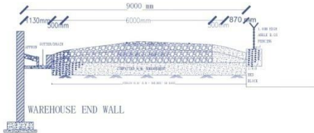
TYPE CROSS SECTION OF ROAD, APPRON, GUTTER/ DRAIN, WIRE FENCING COMPOUND
