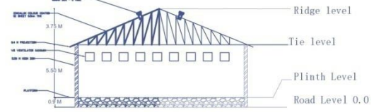
SECTION
