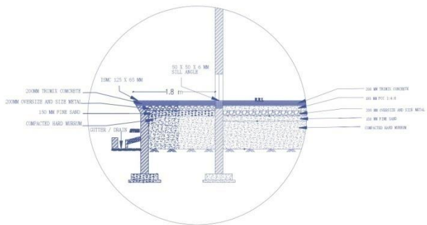
CROSS SECTION PLATFORM
